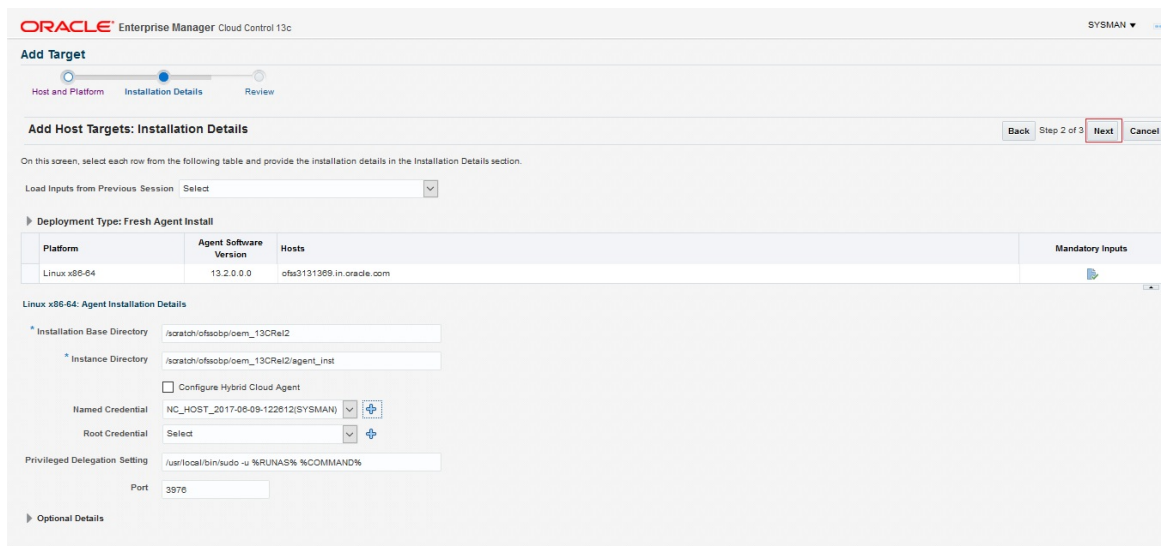
Figure 1–7 Agents Installation Details
