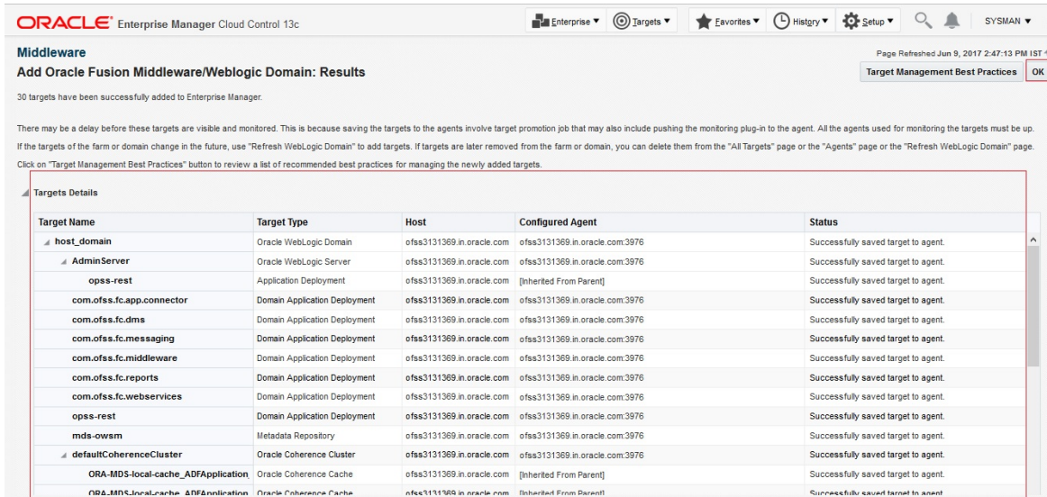
Figure 1–29 Add Oracle Fusion Middleware/Weblogic Domain Results
