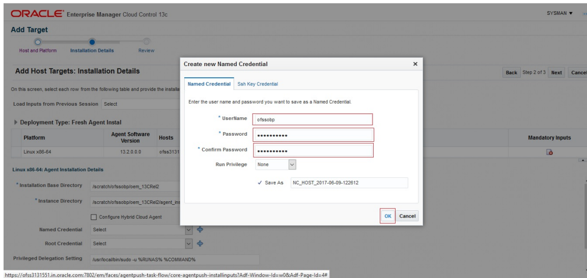
Figure 1–6 Set up Named Credential
